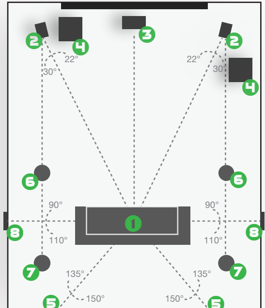
In-room / In-wall / In-ceiling 7.2.4 Speaker Placement
