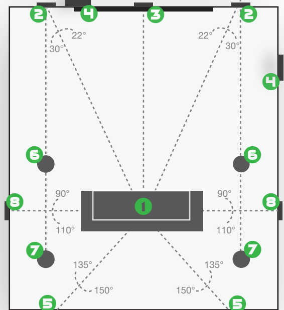
In-wall / In-ceiling 7.2.4 Speaker Placement
