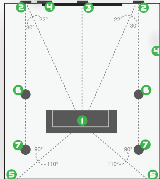
In-wall / In-ceiling 5.2.4 Speaker Placement
