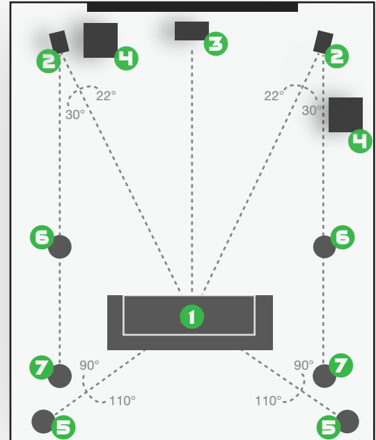
In-room / In-ceiling 5.2.4 Speaker Placement
